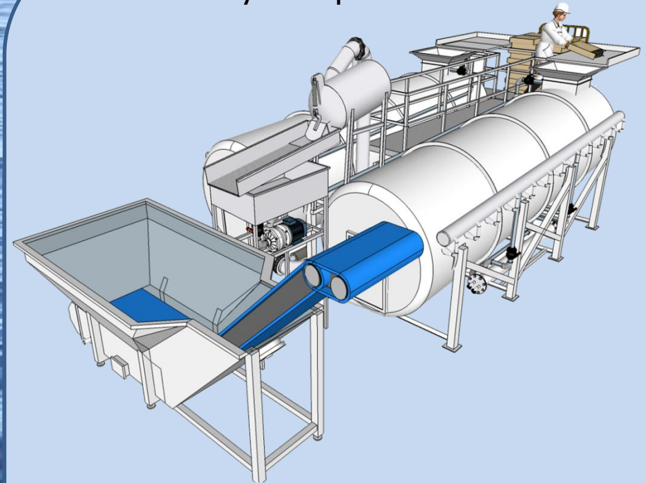
Battery of 2 pcs PTS-LC5
